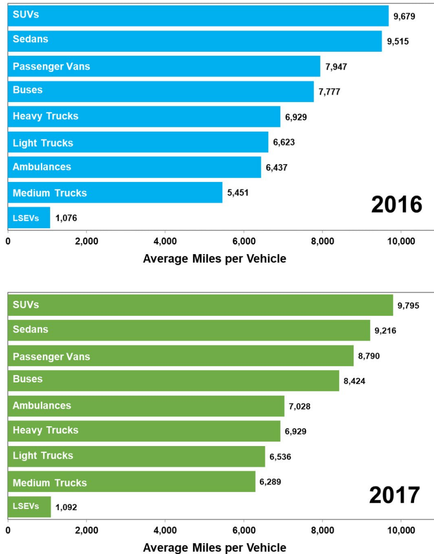
Figure 7.2. Average Miles per Domestic Federal Vehicle by Vehicle Type, 2016 and 2017 (Updated April 2019)
