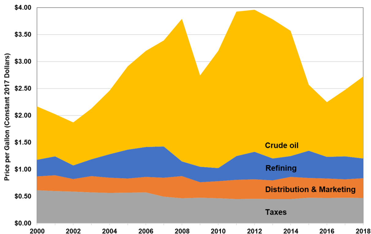
Figure 10.5. Gasoline Price Components, 2000–2018 (Updated April 2019)
