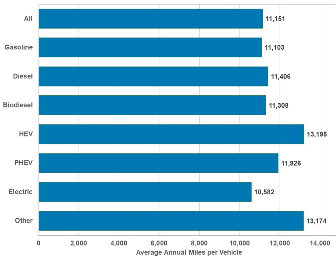
Figure 8.8. Annual Vehicle Miles of Travel by Fuel Type, 2017 NHTS
